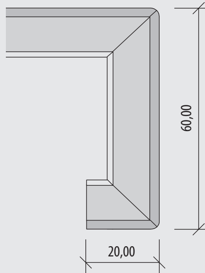
Classic 60
