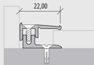
PPS-CHAMPION 287 H
